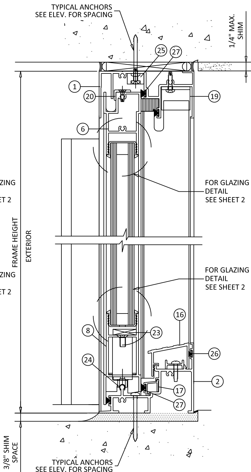
B 4 VERTICAL SECTION OPERABLE PANEL
