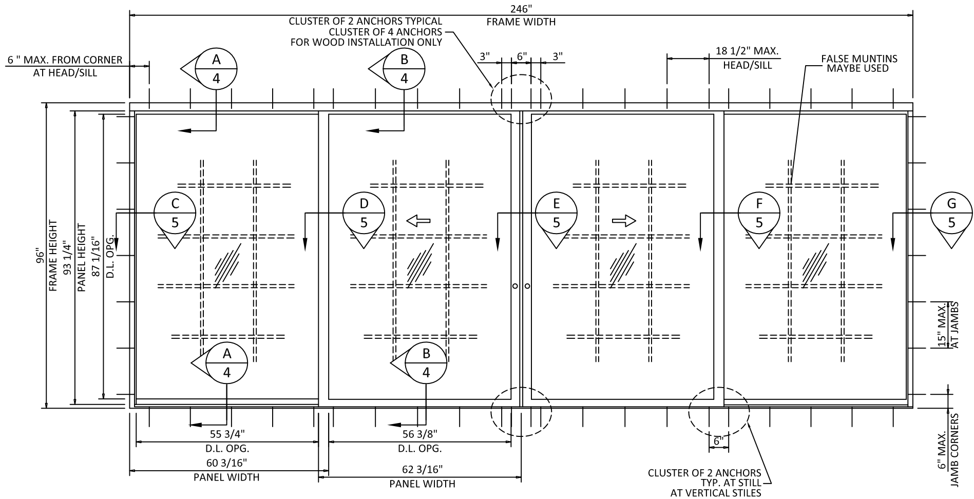
TYPICAL ELEVATION FOR OXO
