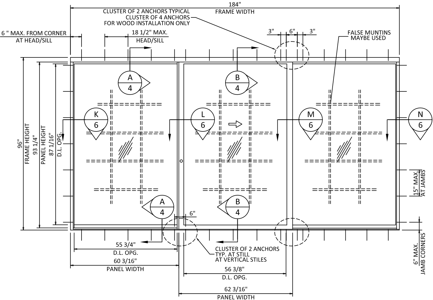
TYPICAL ELEVATION FOR OXO
